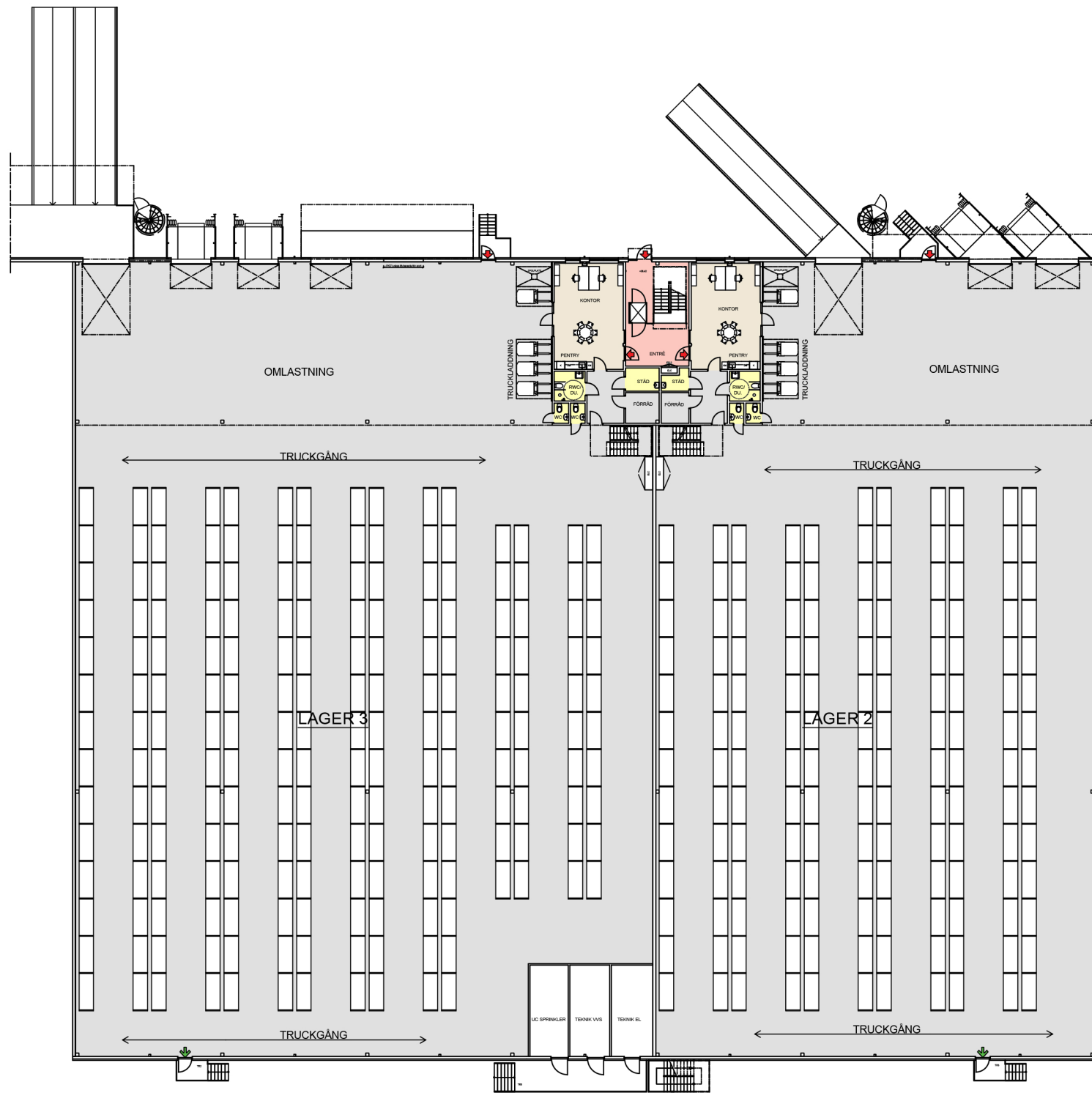
Markplan, Lager Ca 4584 kvm
